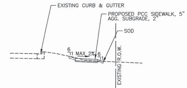
EXISTING & PROPOSED TYPICAL CROSS SECTION (SOUTHEAST CORNER AT PERSHING/ RTE. 53)
