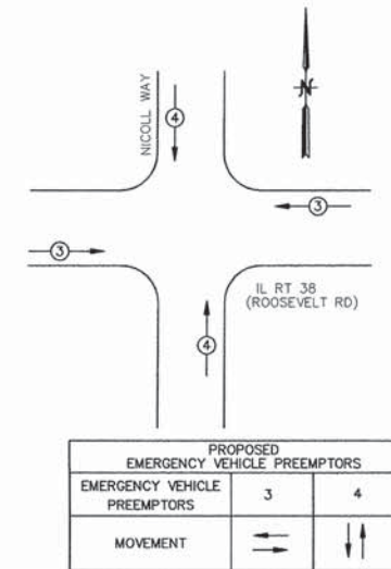
PROPOSED EMERGENCY VEHICLE PREEMPTION SEQUENCE
