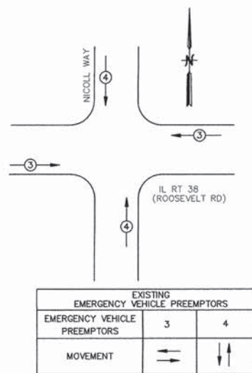
EXISTING EMERGENCY VEHICLE PREEMPTION SEQUENCE
