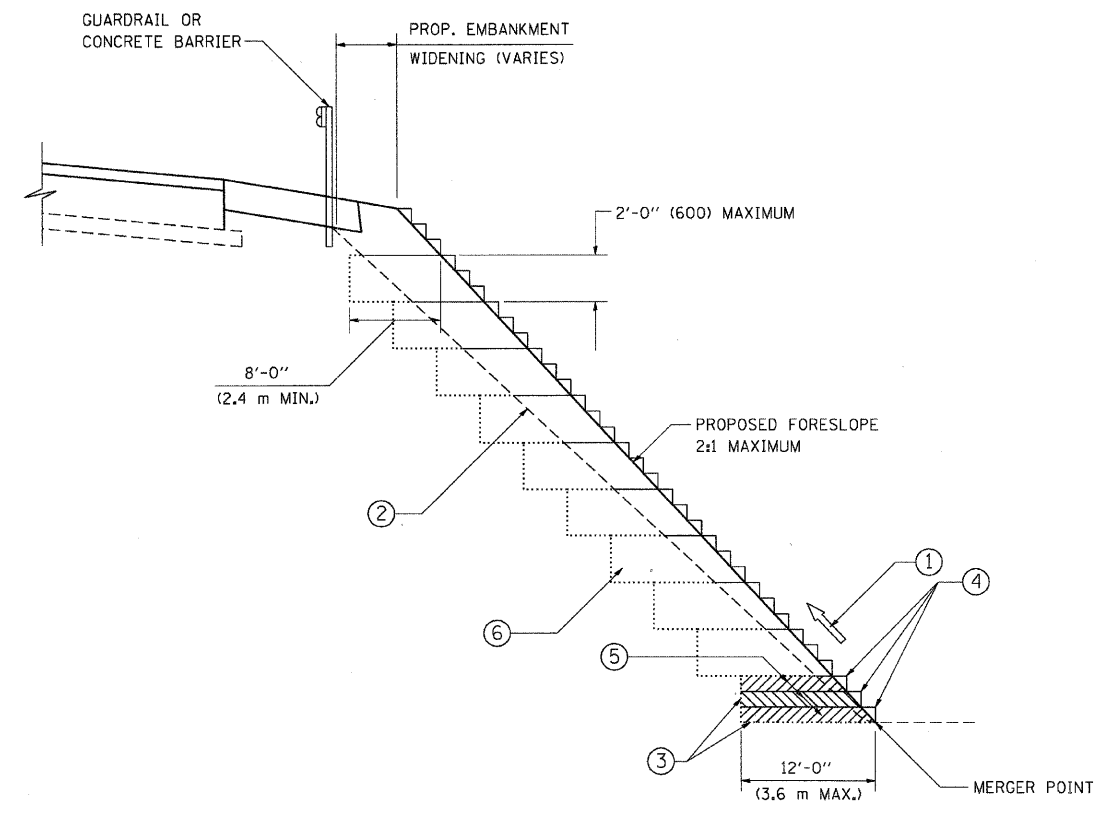
TYPICAL BENCHING DETAIL FOR EMBANKMENT
