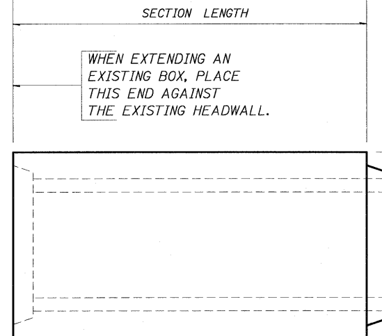
PLAN LOCATION OF LIFTING HOLES MAY BE VARIED AS NEEDED TO CLEAR REINFORCEMENT.
