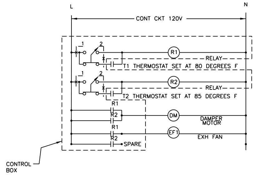
4 ELECTRICAL ROOM EXHAUST FAN CONTROL DIAGRAM SCALE N/A
