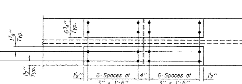
INSIDE FLANGE SPLICE
