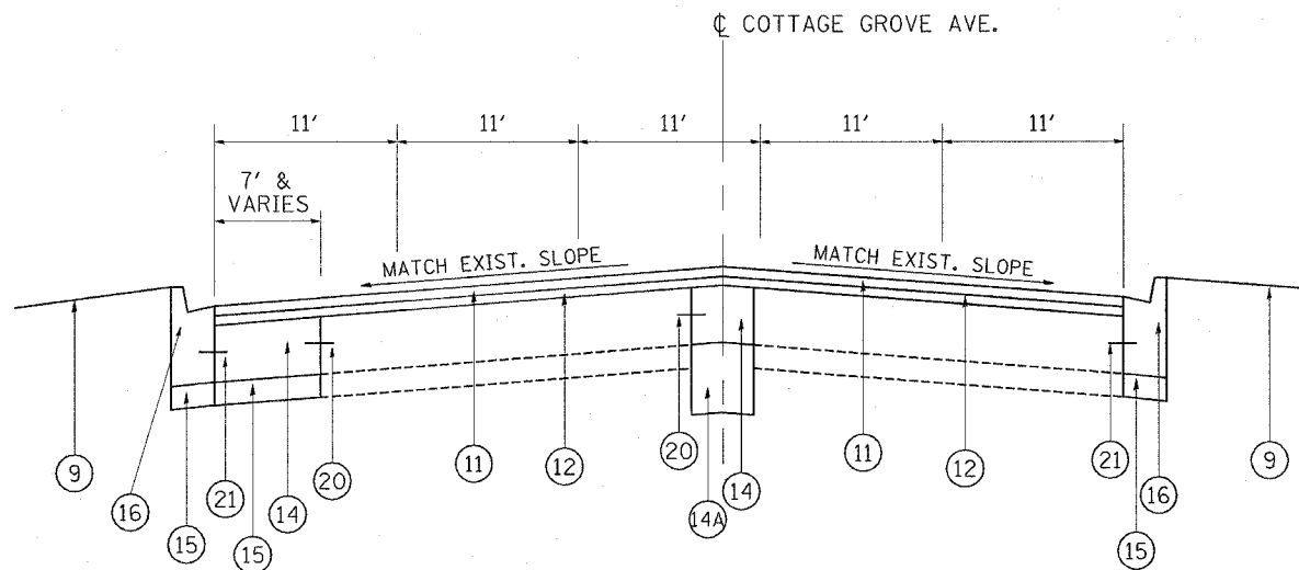
PROPOSED TYPICAL SECTION COTTAGE GROVE AVE. STA. 113+80 TO 116+20
