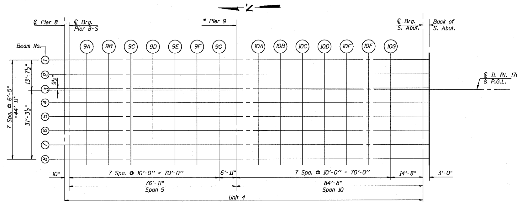
PLAN (UNIT 4)
