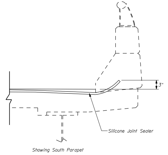
TYPICAL END OF SEAL TREATMENT
