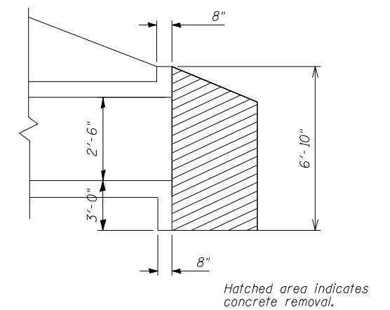
EXISTING OUTLET
