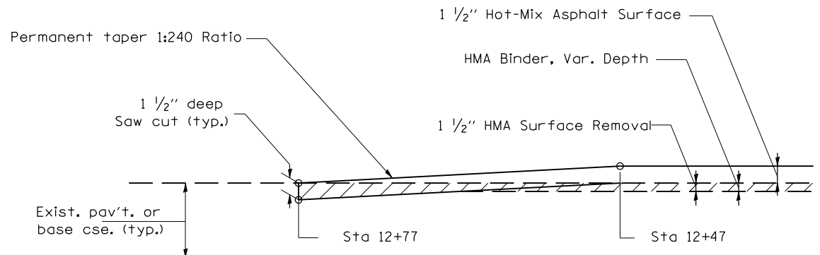
BUTT JOINT DETAIL FRANKLIN ST. (NORTH)
