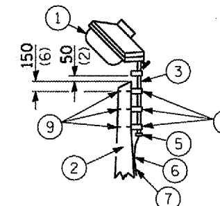
TENON
