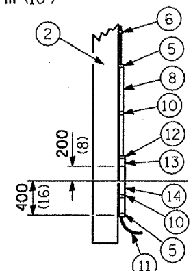
POLE, WOOD
