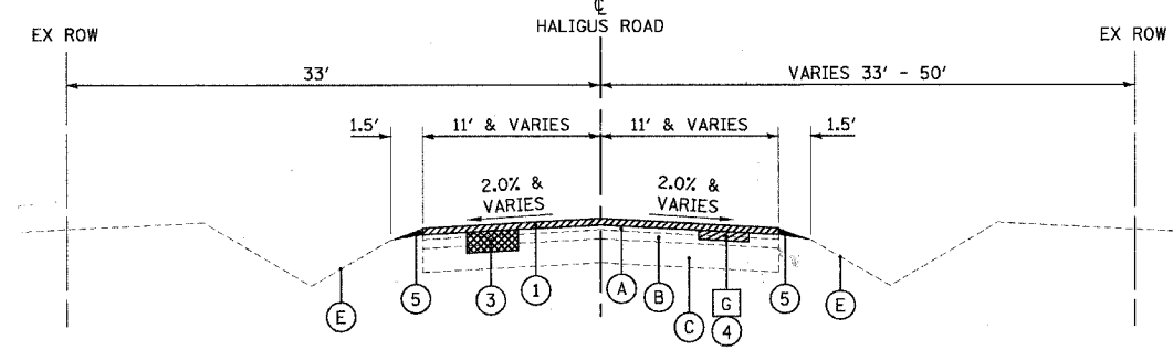
PROPOSED TYPICAL SECTION HALIGUS ROAD STA. 9+20 TO STA. 32+50
