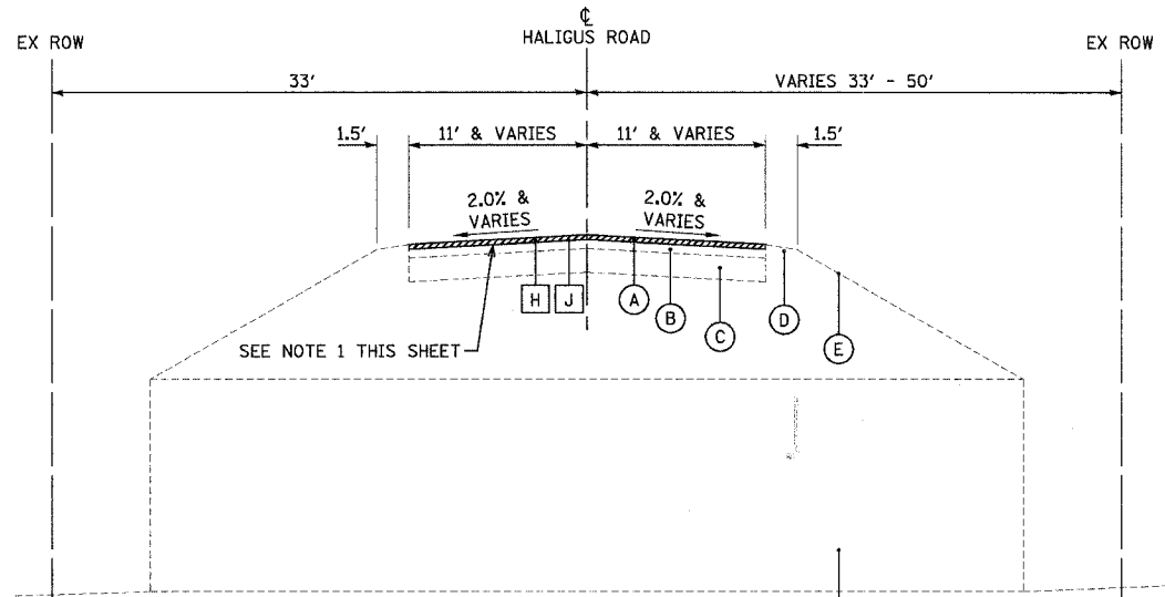
EXISTING TYPICAL SECTION HALIGUS ROAD STA. 48+00 TO STA. 52+00
