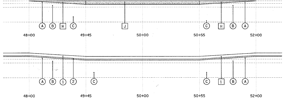
HOT-MIX ASPHALT SURFACE REMOVAL AND RESURFACING
