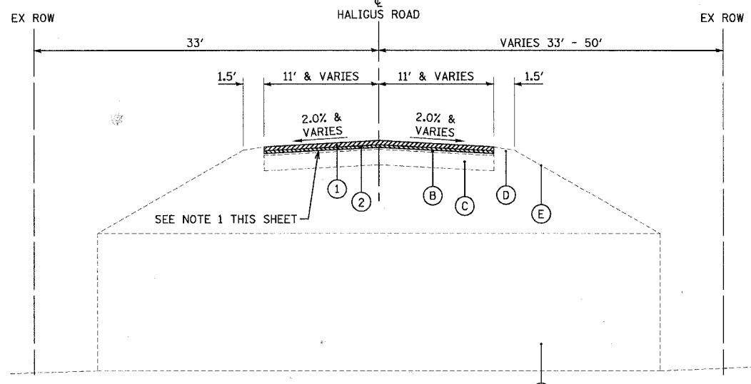
PROPOSED TYPICAL SECTION HALIGUS ROAD STA. 48+00 TO STA. 52+00
