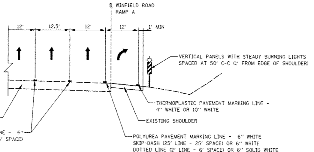
TYPICAL SECTION
