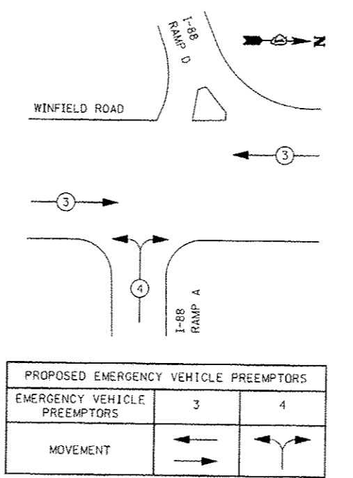
EMERGENCY VEHICLE PREEMPTION SEQUENCE ALL STAGES
