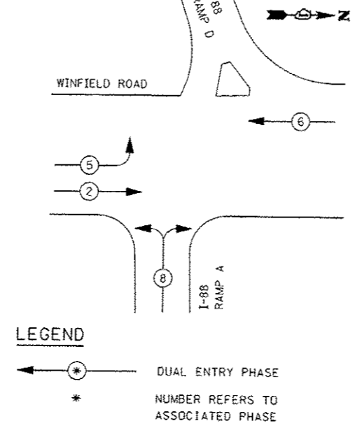
TEMPORARY PHASE DESIGNATION DIAGRAM ALL STAGES
