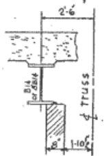
SECTION A-A scale 3/4" = 1'-0"
