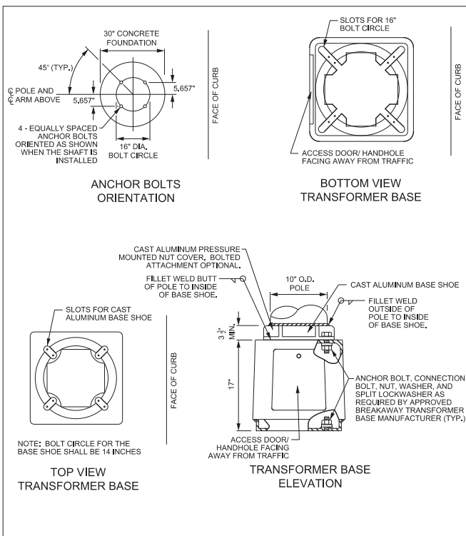
DETAIL "C" - BREAKAWAY TRANSFORMER BASE FOR ROADWAY LIGHTING NOT TO SCALE
