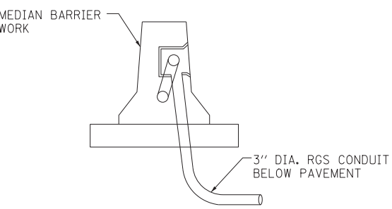
JUNCTION BOX EMBEDDED IN CONCRETE BARRIER N.T.S.
