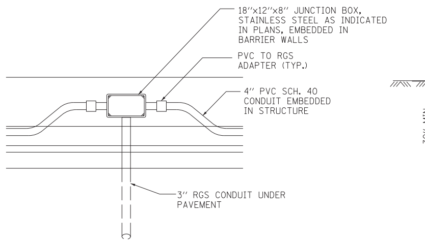
SINGLE DUCT BANK DETAIL N.T.S.
