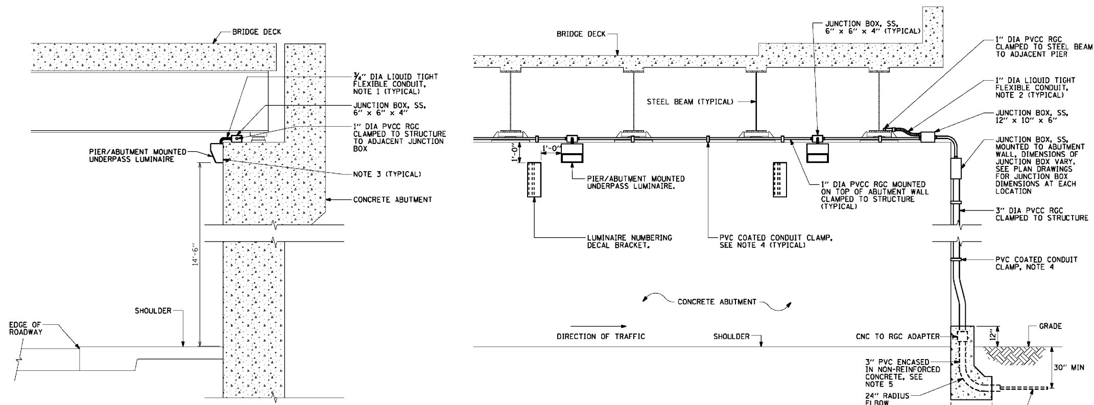
TYPICAL PIER / ABUTMENT MOUNTED UNDERPASS LIGHTING INSTALLATION DETAILS
