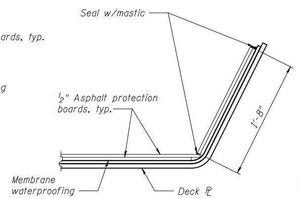
WATERPROOFING AT DECK PLATE
