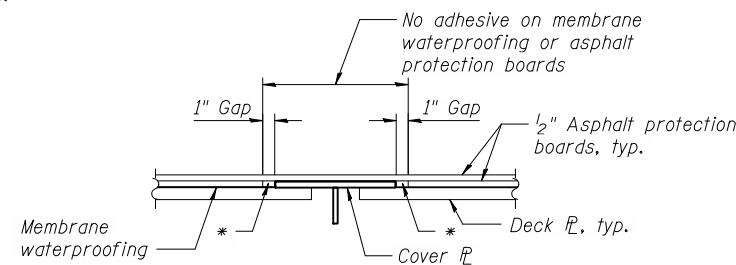
WATERPROOFING AT COVER PLATE
