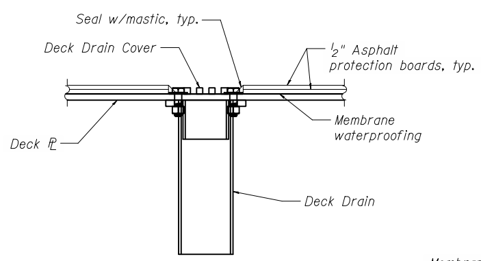
WATERPROOFING AT DECK DRAIN
