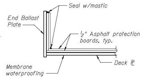
WATERPROOFING AT END BALLAST PLATE
