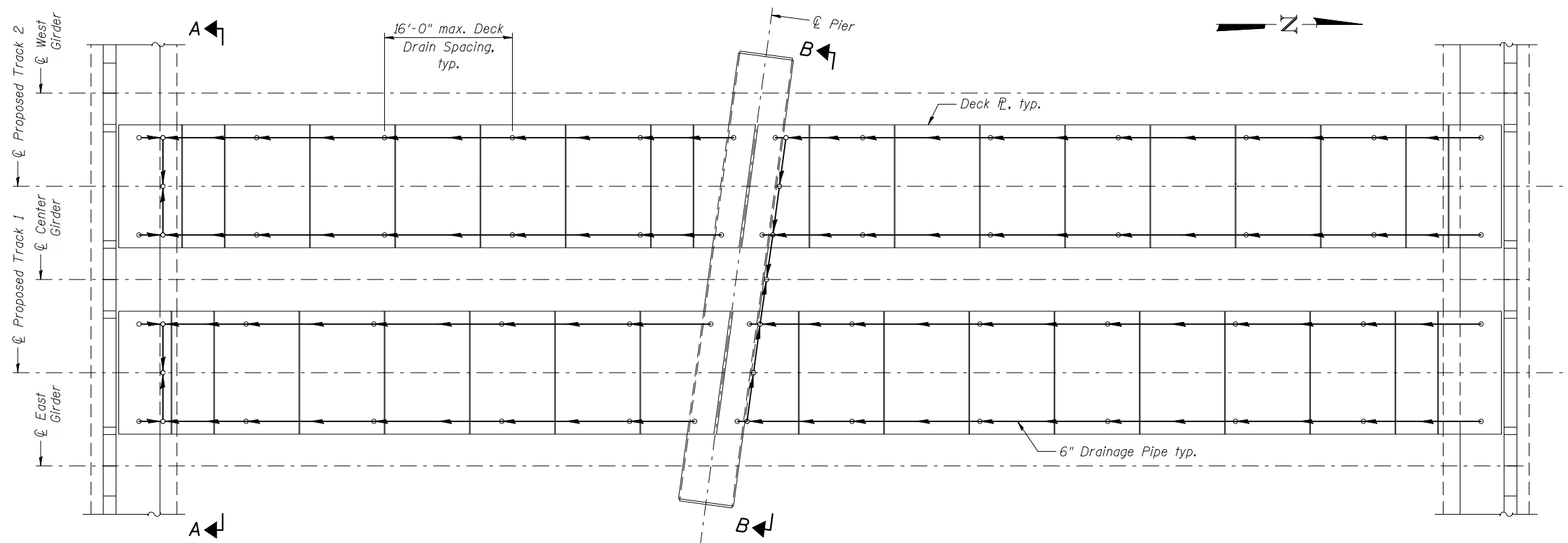
DECK DRAINAGE PLAN
