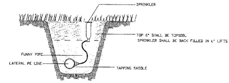
3 SPRAY HEAD AND SMALL ROTOR HEAD NO SCALE
