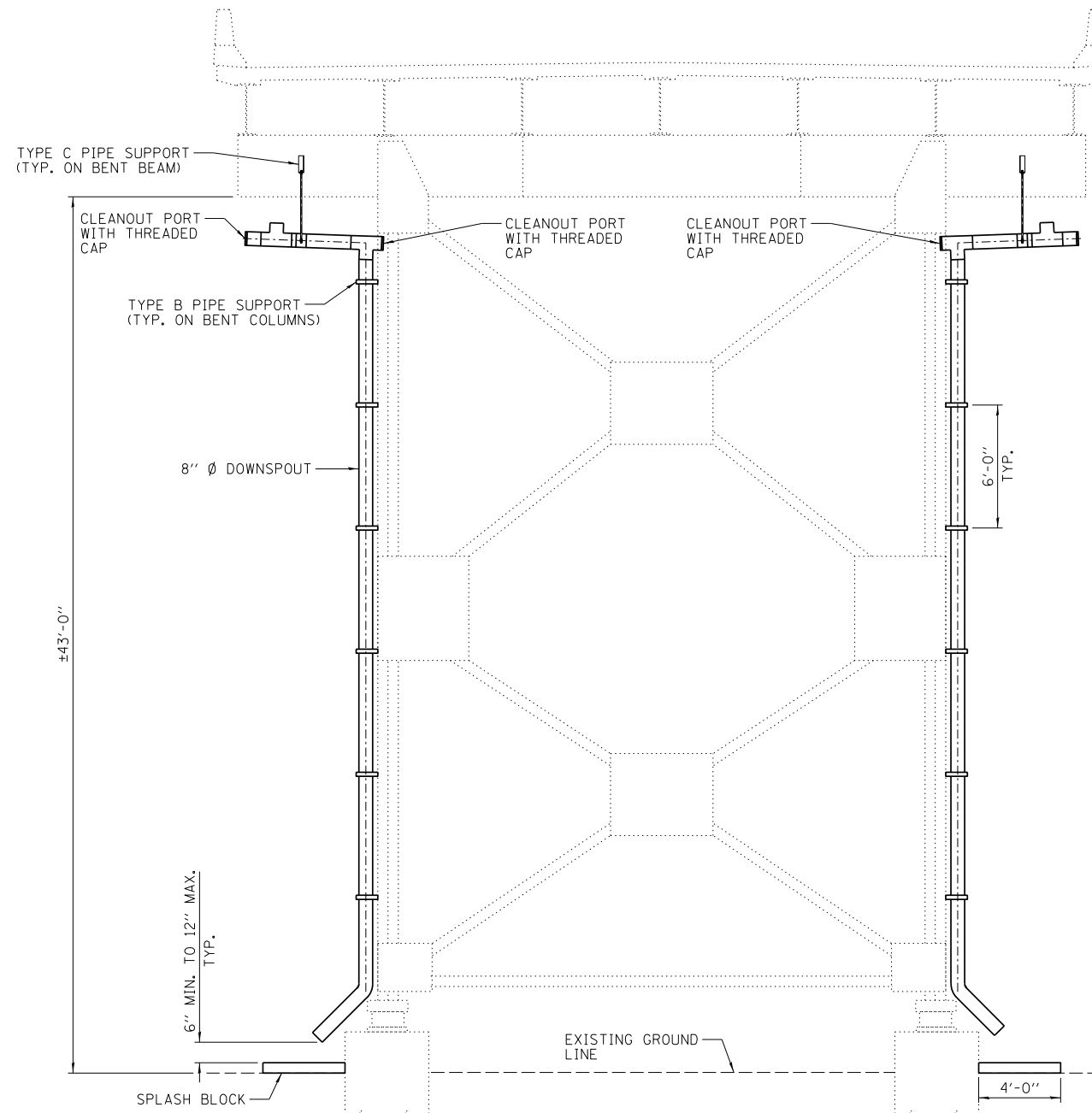
DRAINAGE SYSTEM ELEVATION AT BENT 33 (LOOKING WEST/S.N. 082-6003)
