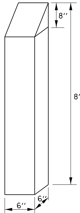
WOOD BLOCK PRESSURE TREATED
