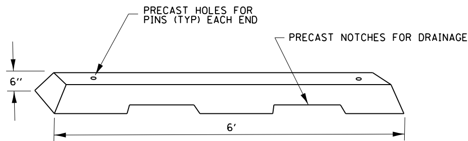
6' CONCRETE PARKING CURB
