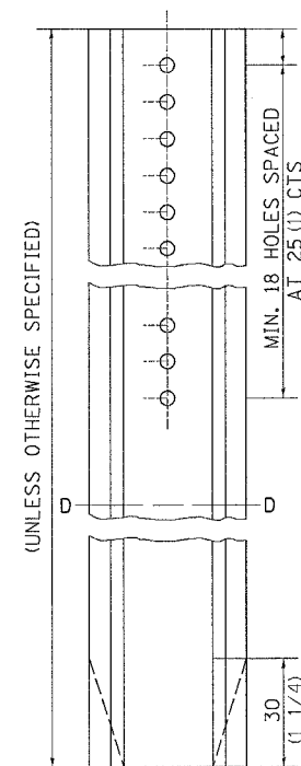
DELINEATOR AND POST ORIENTATION
