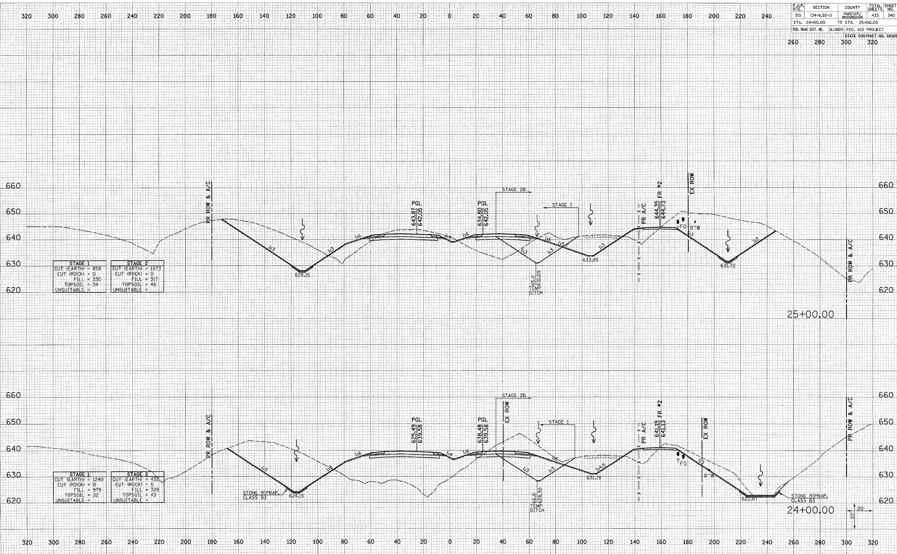
FAP ROUTE 315 (IL 336) CROSS SECTIONS STA 24+00.00 TO 25+00.00
