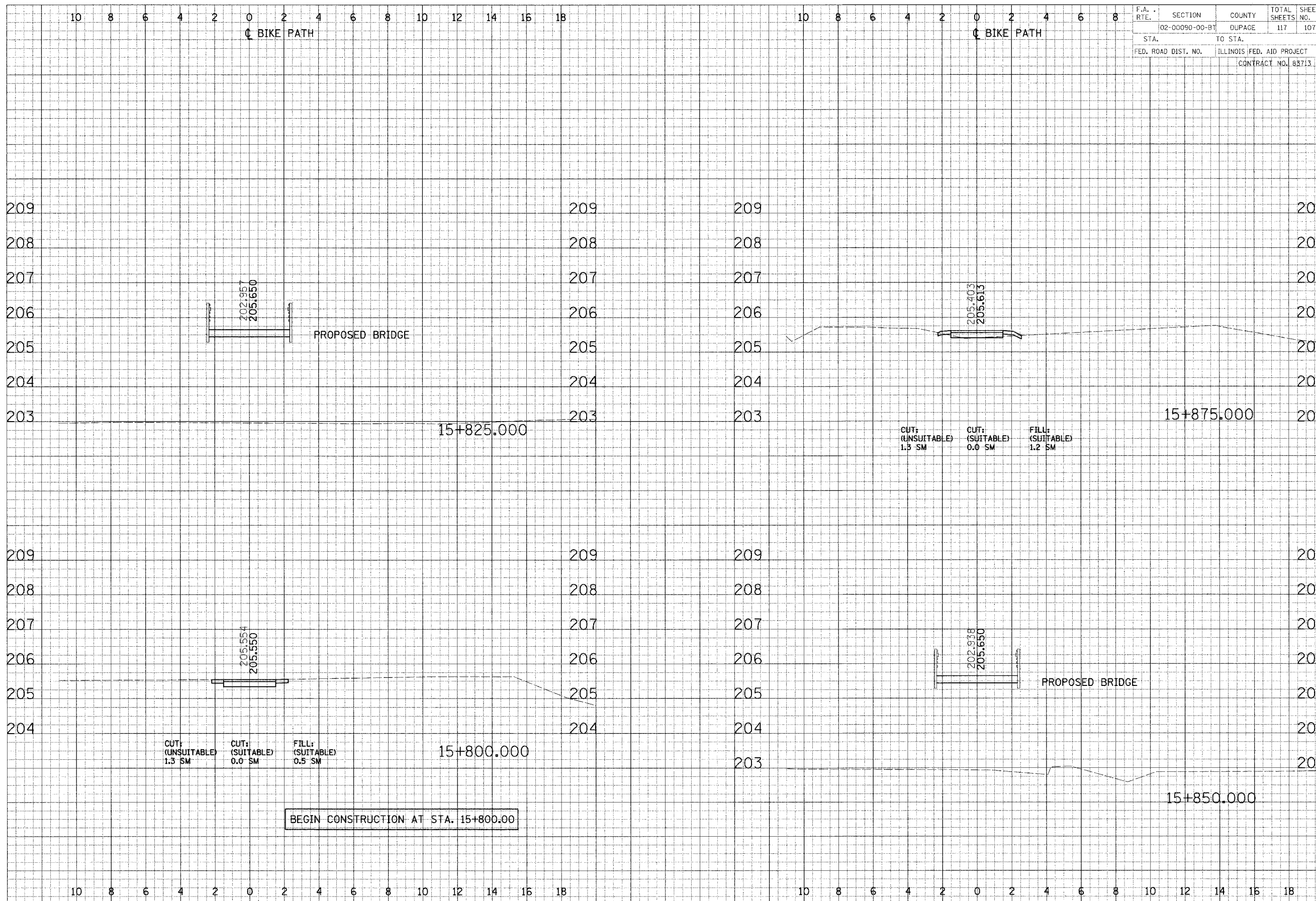
CROSS SECTIONS - NORTH AVE
