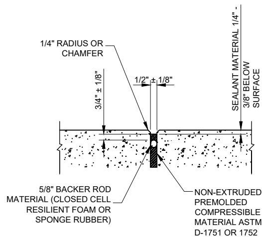
DETAIL 1 - SEALANT
