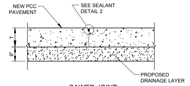
SAWED JOINT
