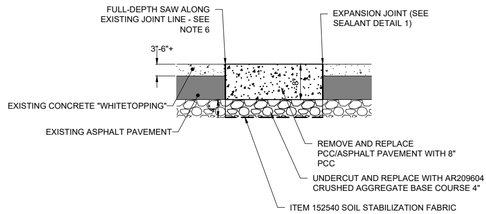
PAVEMENT PATCHING DETAIL NOT TO SCALE
