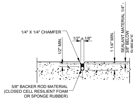
DETAIL 2 - SEALANT
