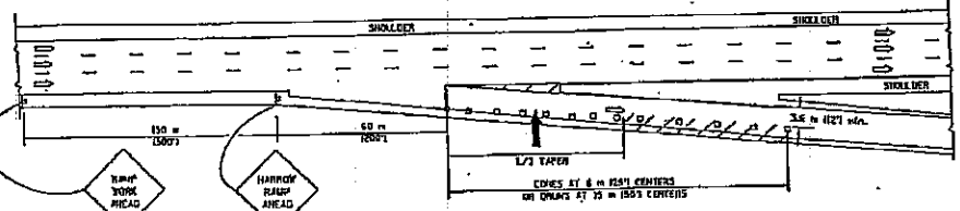
TYPICAL EXIT RAMP
