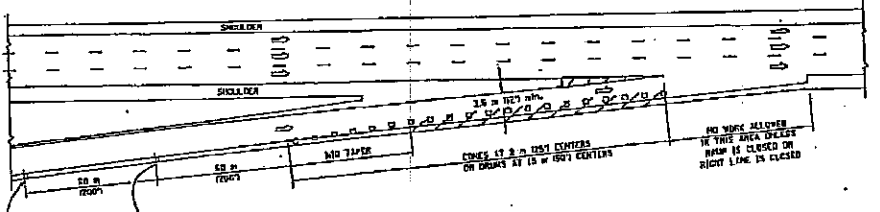
TYPICAL ENTRANCE RAMP
