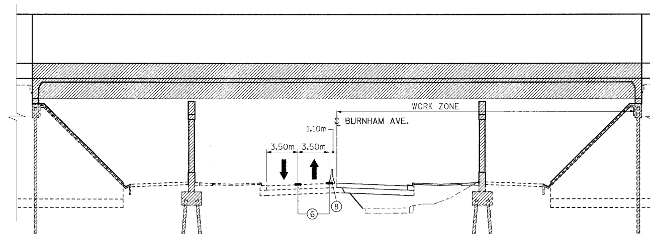
TYPICAL SECTION (STAGE II) STA 59+971.200 TO STA 60+030.745
