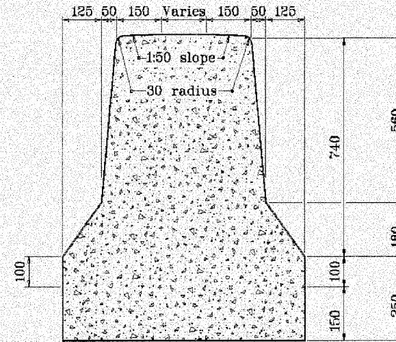
SECTION E-E
