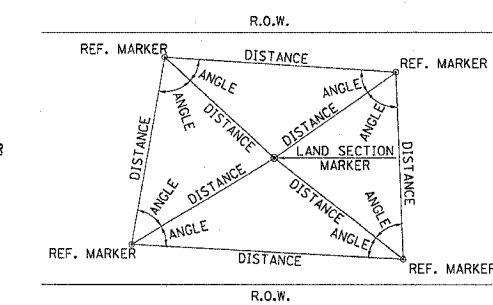
SECTION CORNER TIE POINT CAP
