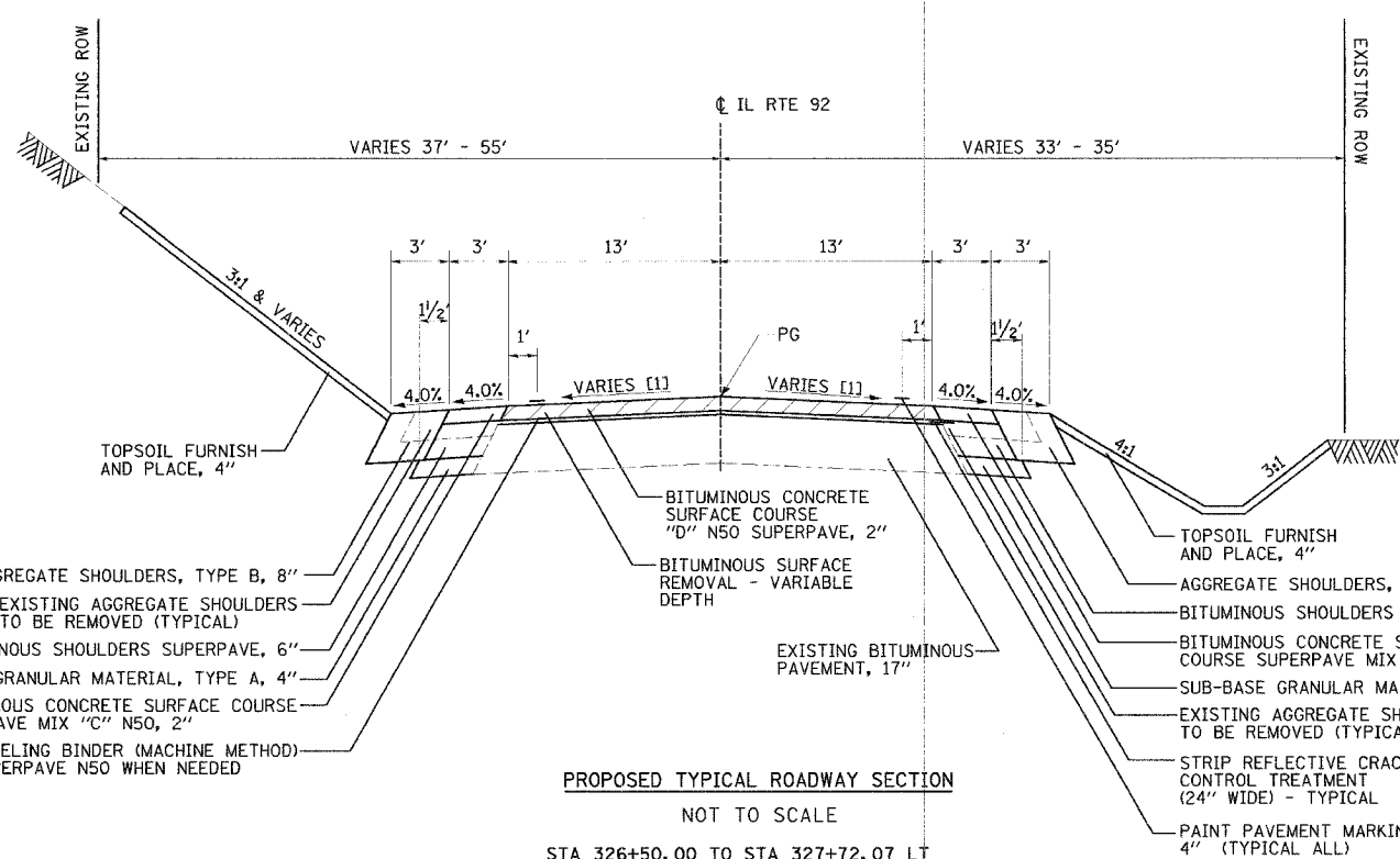
EXISTING TYPICAL ROADWAY SECTION NOT TO SCALE STA 326+50.00 TO STA 336+10.00
