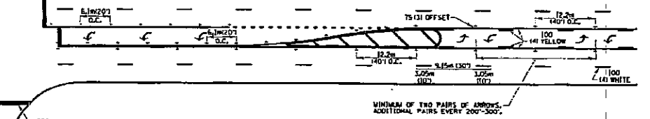
TYPICAL PAVEMENT MARKING FOR TWO LANE SECTION - NO PASSING ZONES
