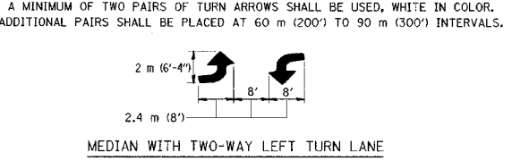
TYPICAL LEFT (OR RIGHT) TURN LANE MARKING
