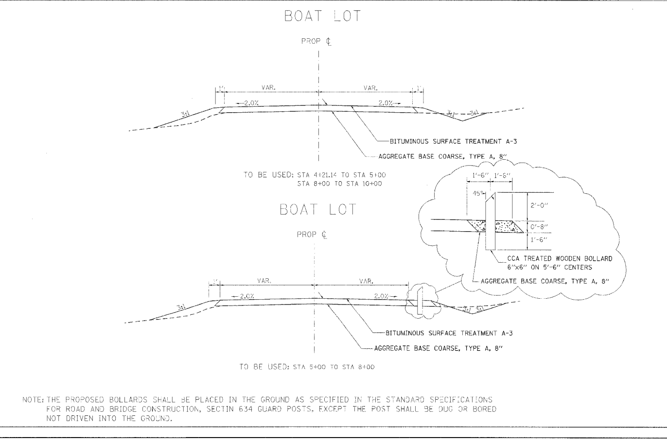
PLAN PROFILE, TYPICAL, & BOLLARD DETAIL BOAT LOT STA 4+21.14 TO 10+00
