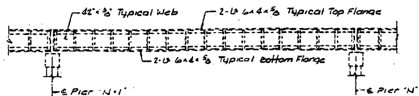
GIRDER ELEVATION
