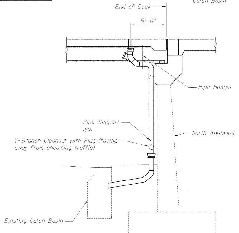
ELEVATION AT NORTH ABUTMENT (Looking North)
