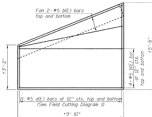
WIDENED APPROACH SLAB DETAIL
