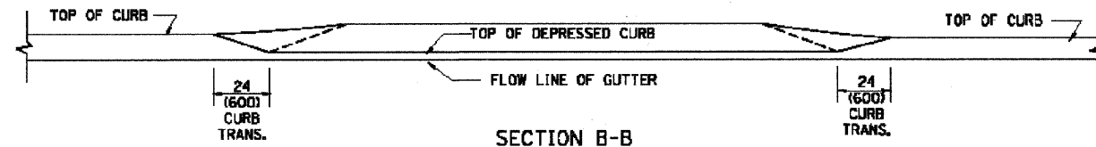
SECTION B-B
