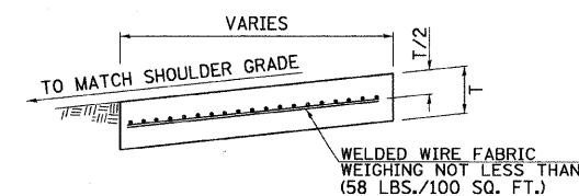
SECTION C-C
