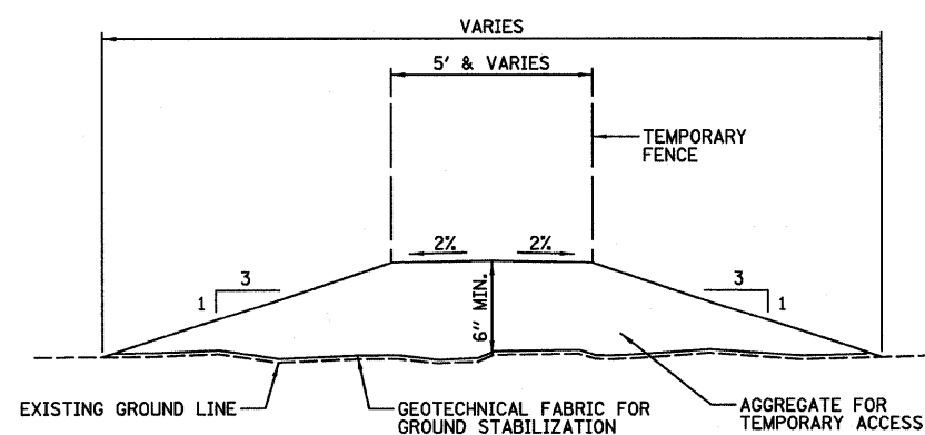
TEMPORARY TRAIL CROSS SECTION
