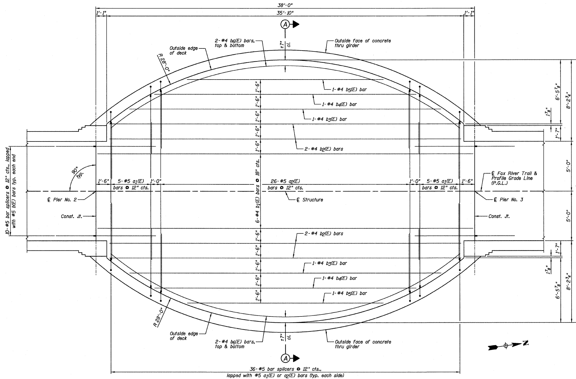
REINFORCEMENT STEEL PLAN
