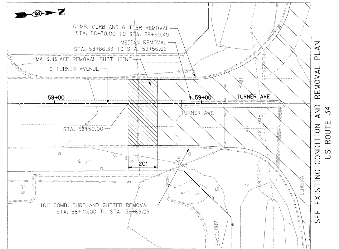
EXISTING CONDITION AND REMOVAL PLAN TURNER AVENUE
