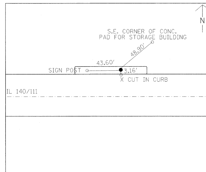
CONTROL PT 504 REBAR WITH IDOT CAP STA. 471+94.98 38.62 LT N 814,941.84 E 322,117.17
