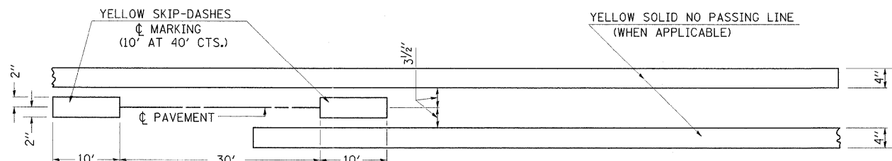
TYPICAL SPACING
