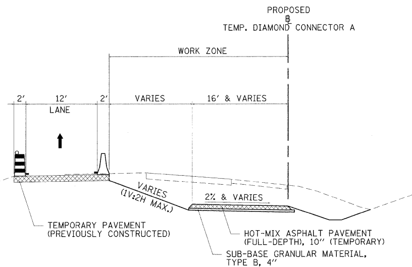
RAMP A - PRE-STAGE B TYPICAL #1 TEMP. DIAMOND CONNECTOR A: STA. 13+75.00 TO STA. 19+65.71
