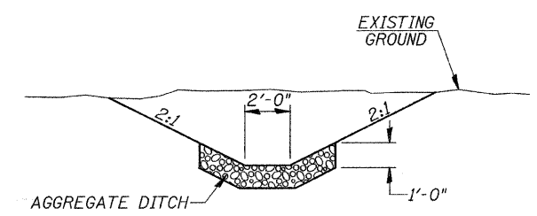
DETAIL OF CULVERT OUTLET DITCH AT 15+50 RT.
