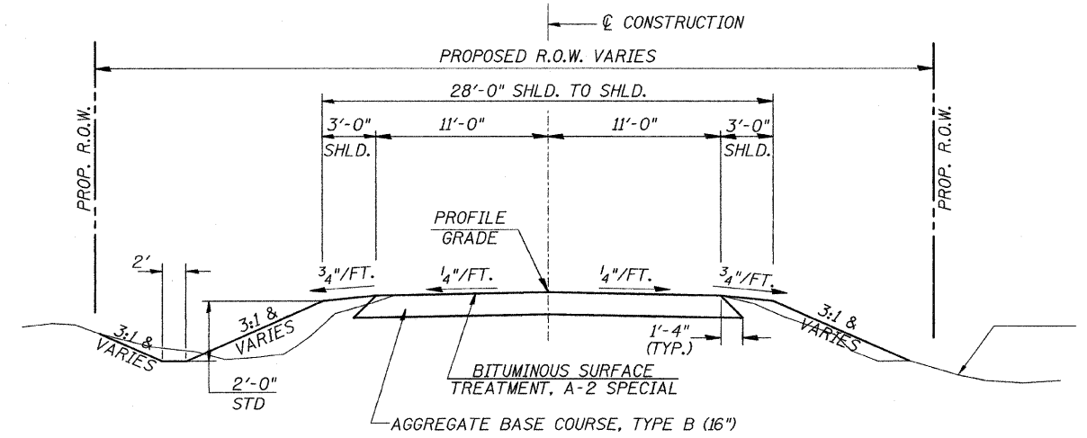
PROPOSED TYPICAL SECTION STA. STA. 15+00.00 TO STA. 19+73.50 STA. 20+26.50 TO STA. 25+00.00 BRIDGE OMISSION STA. 19+73.50 TO STA. 20+26.50
