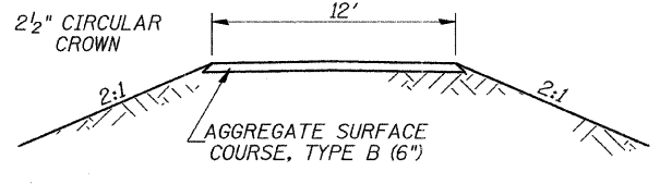
PROPOSED PRIVATE ENTRANCE STA 18+85 LT
