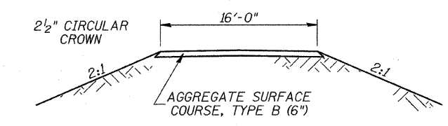
PROPOSED FIELD ENTRANCES STA 18+13 LT STA 21+26 RT
