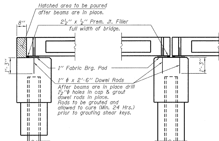
SECTION AT ABUTMENTS
