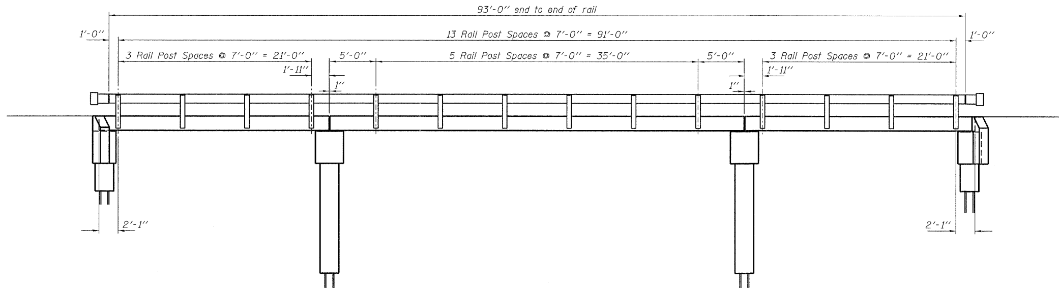
ELEVATION Showing Rail Post Spaces See sheet 7 of 12 for Railing Details.
