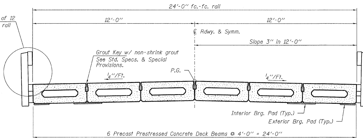
CROSS SECTION See sheets 2 thru 5 of 12 for Superstructure.
