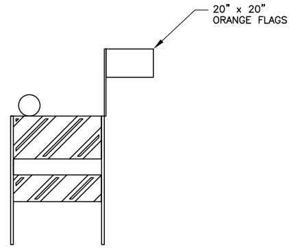
FLASHER BARRICADE DETAIL-IDOT TYPE 2
