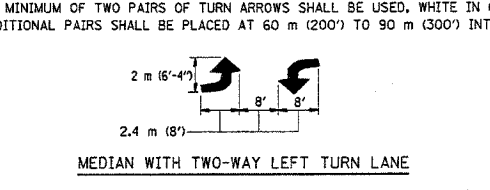
TYPICAL PAINTED MEDIAN MARKING
