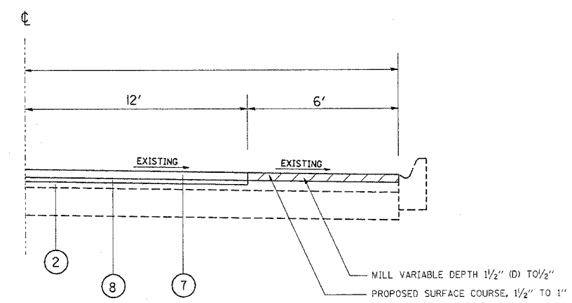
EXIST. AND PROP. PARKING LANE TYPICAL SECTION
